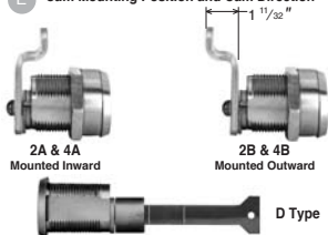
2A&2B Offset Cam Fixed Motion
